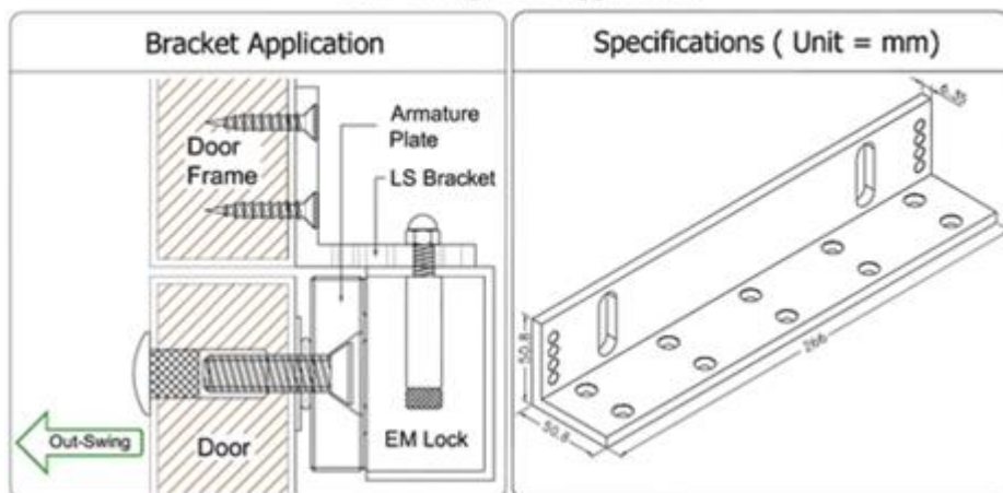
Out - Swing Door Application
